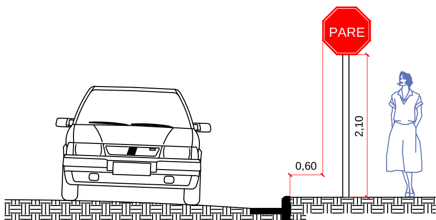
VISTA FRONTAL
